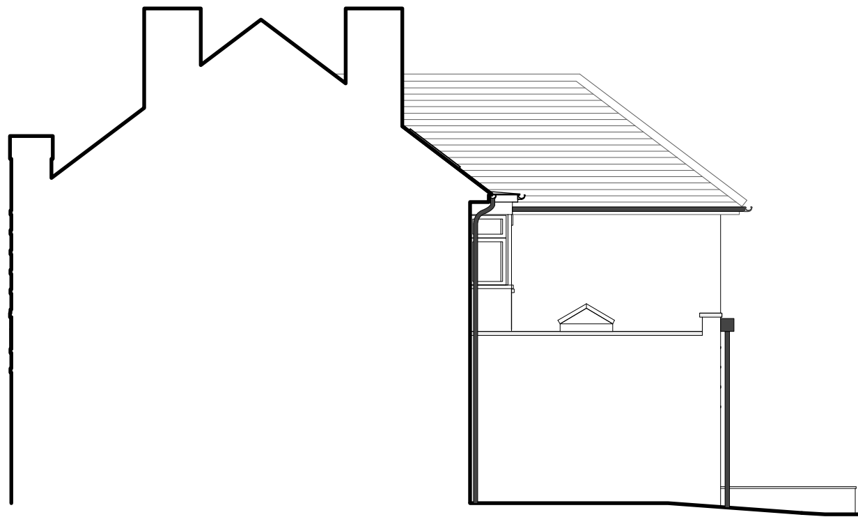
NORTH EAST SIDE ELEVATION (PARTYWALL)
