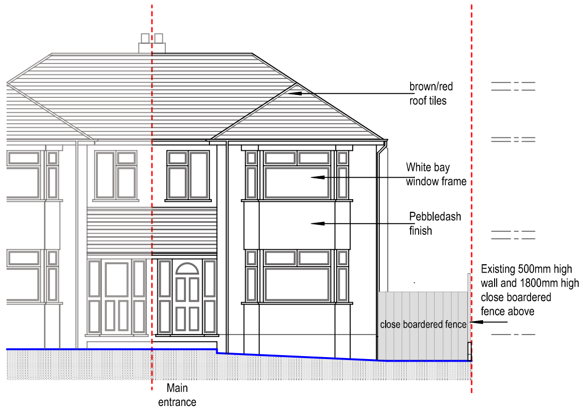
FRONT ELEVATION
