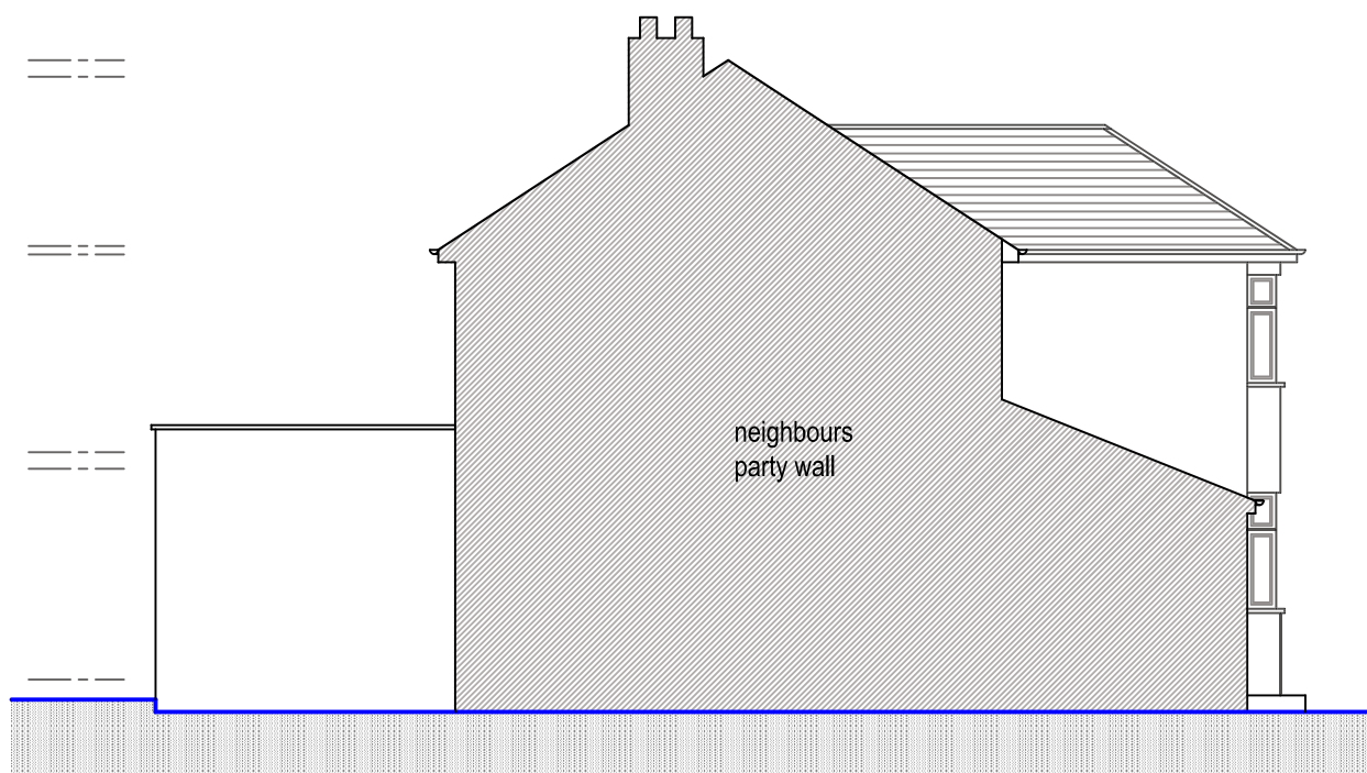
SIDE ELEVATION
