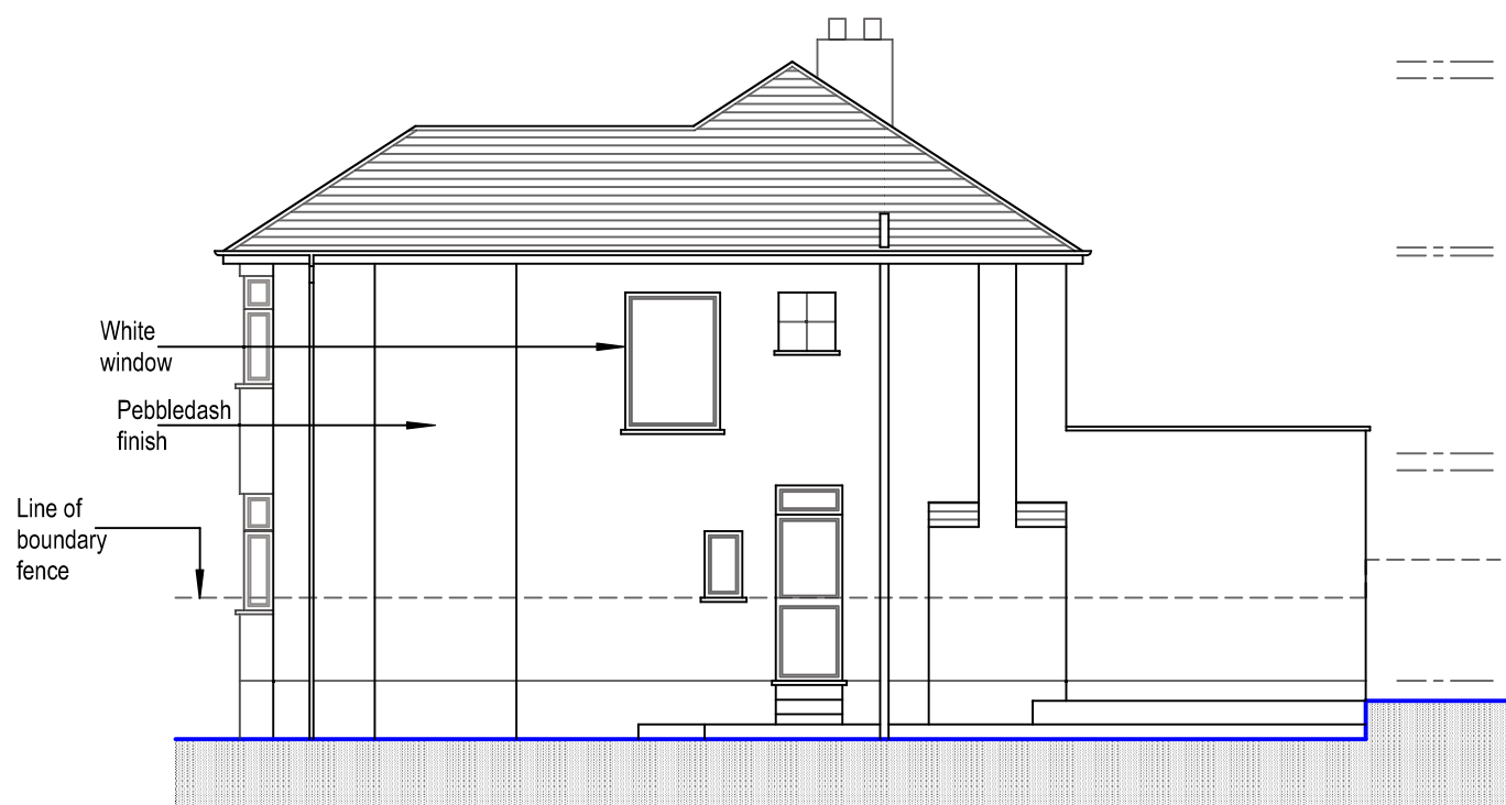
SIDE ELEVATION
