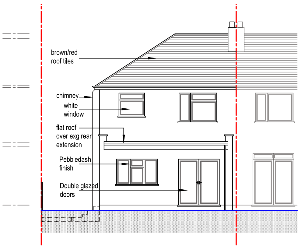
REAR ELEVATION
