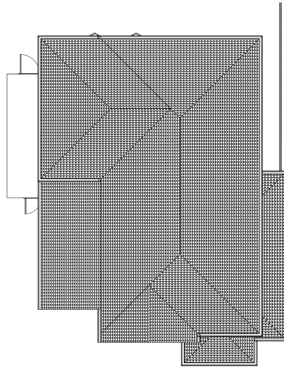
Roof - Proposed 1 : 100
