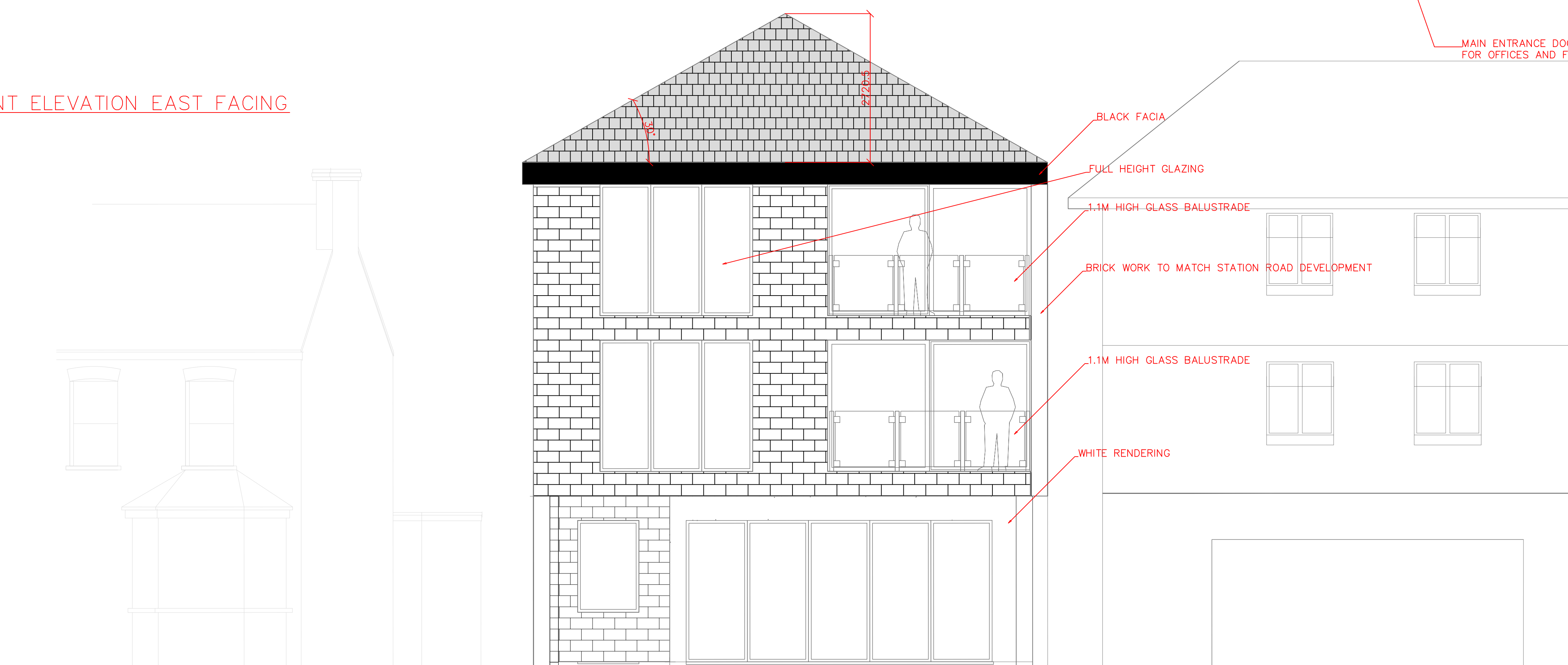
FRONT ELEVATION EAST
