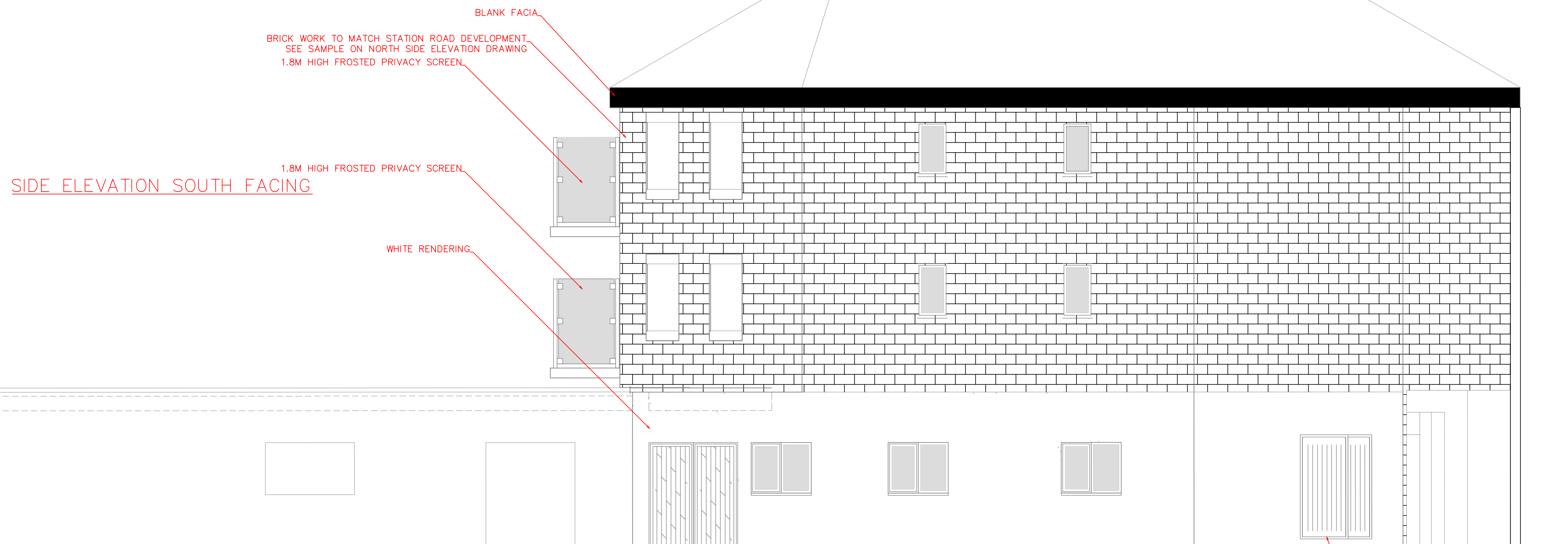
SIDE ELEVATION SOUTH
