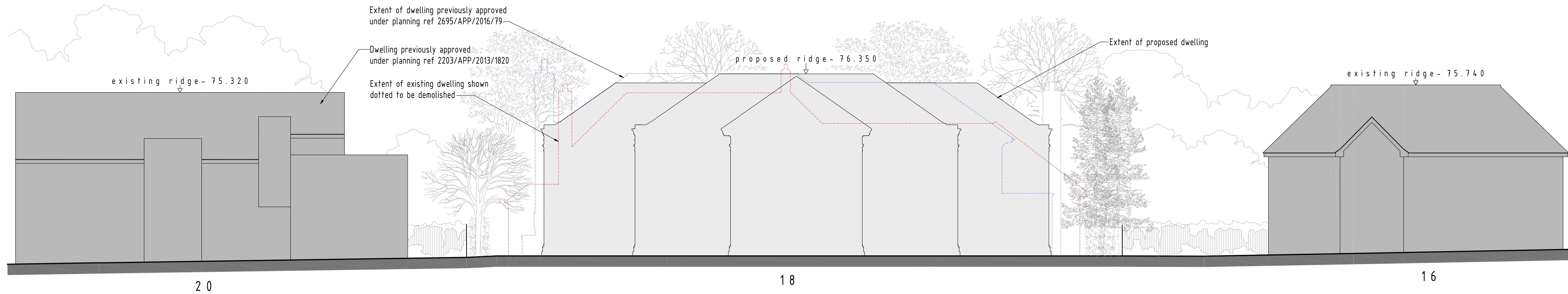
SITE SECTION COMPARISON THROUGH FRONTAGE SCALE 1:100
