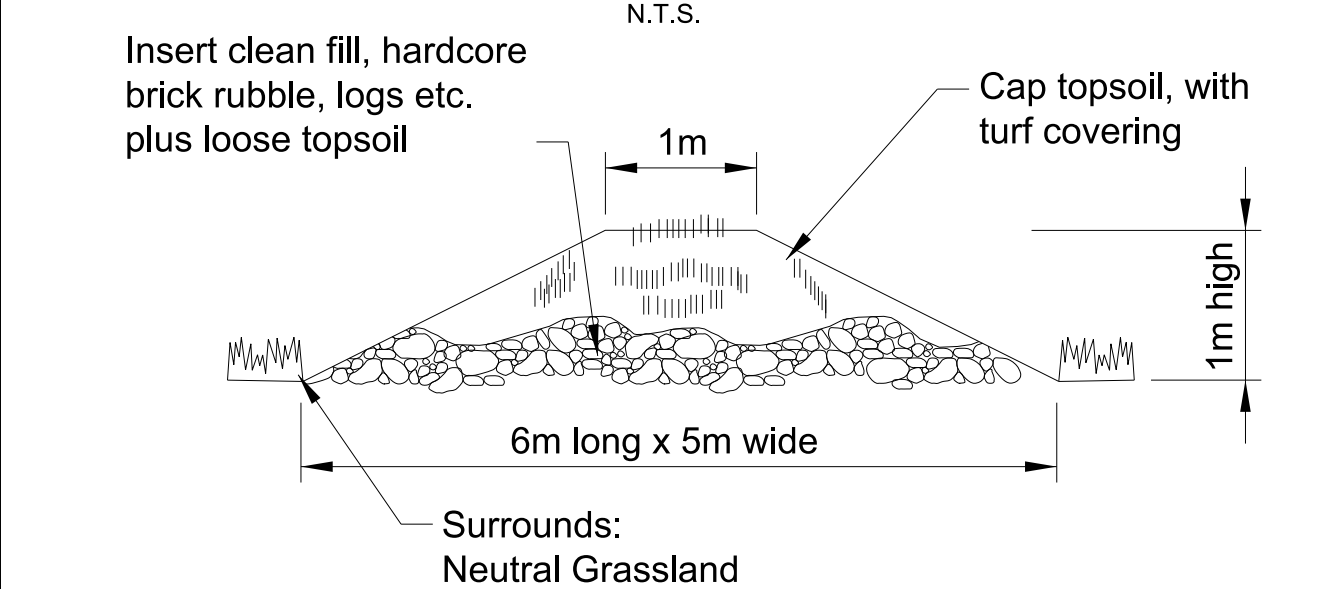
TYPICAL HIBERNACULA CROSS SECTION
