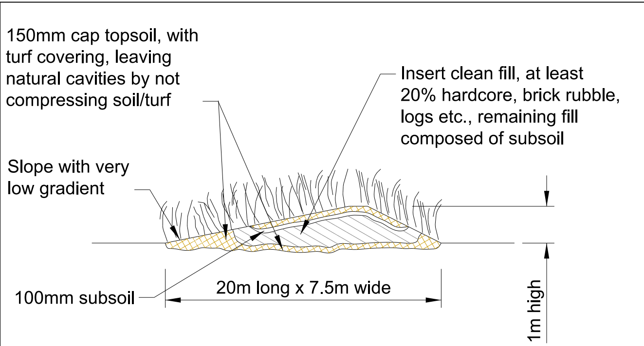
TYPICAL REPTILE BASKING BANK CROSS SECTION
