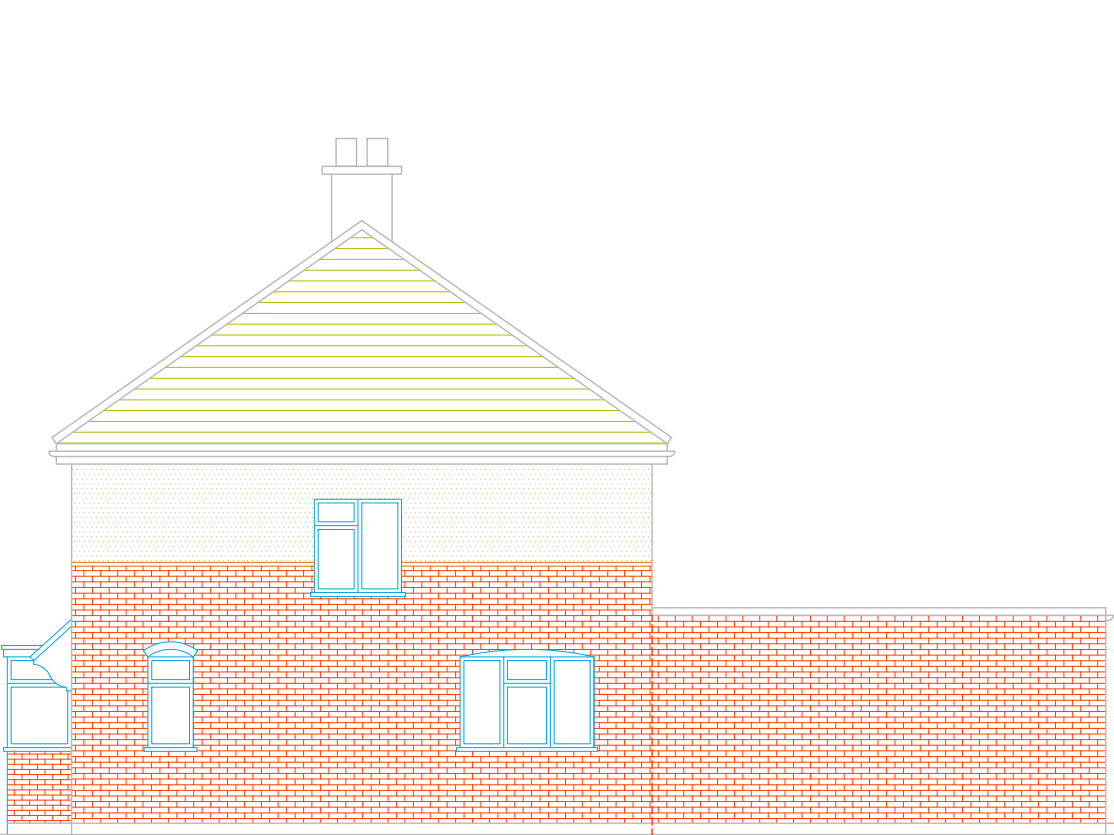
PROPOSED SIDE ELEVATION-1
