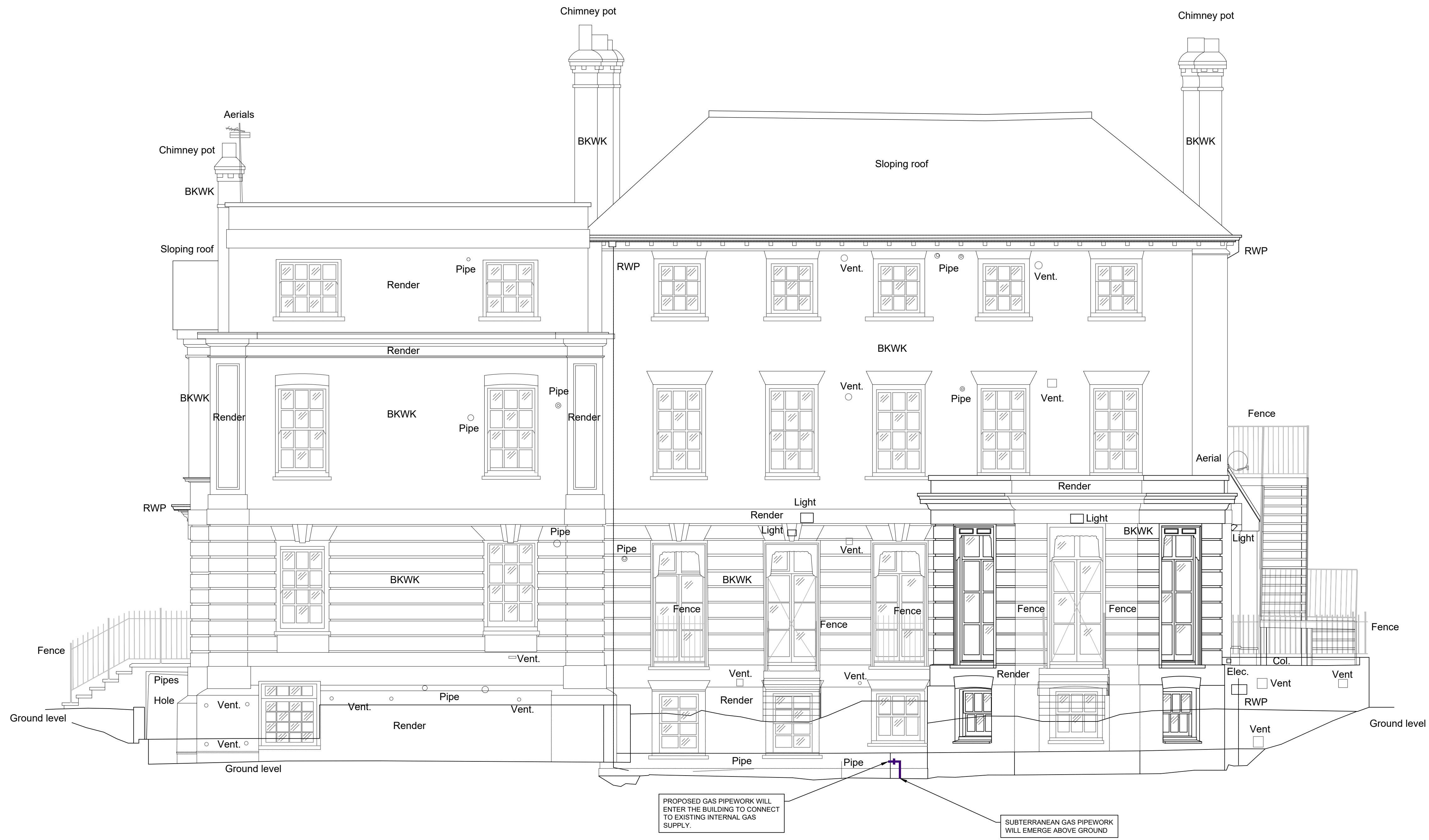
Datum 30.00m West Facing (Rear) Elevation
