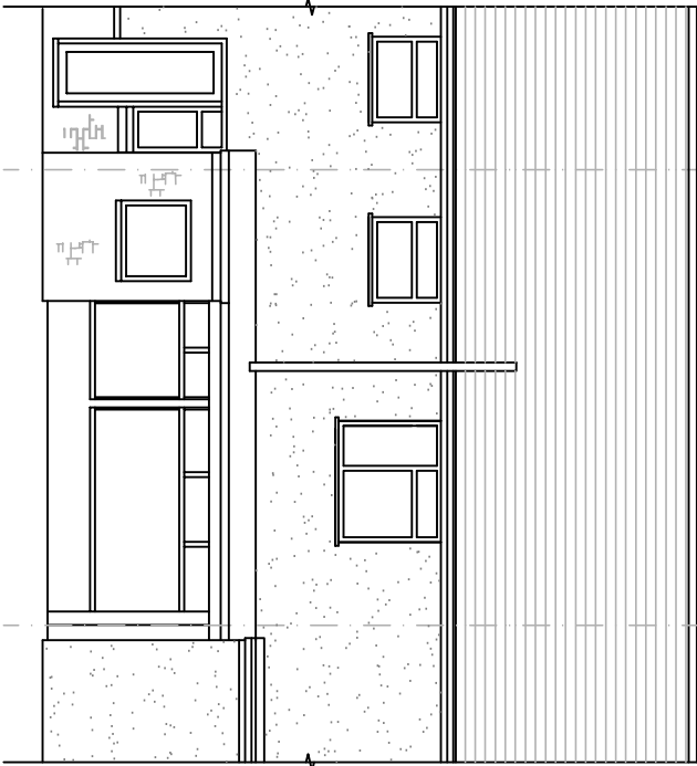
SOUTH-EAST ELEVATION
