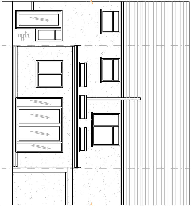
SOUTH-EAST ELEVATION
