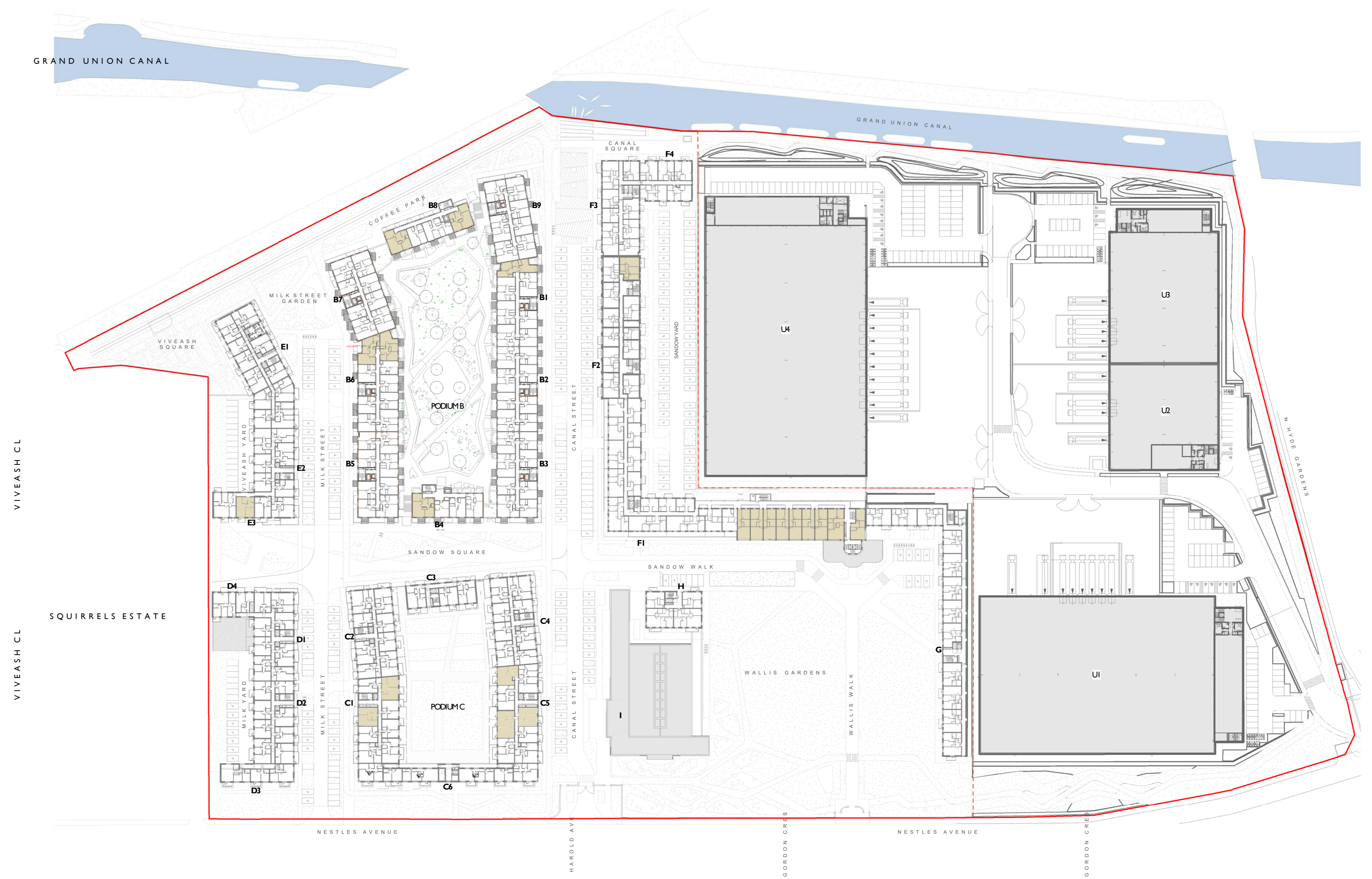
ACCESSIBLE UNITS - THIRD FLOOR PLAN
