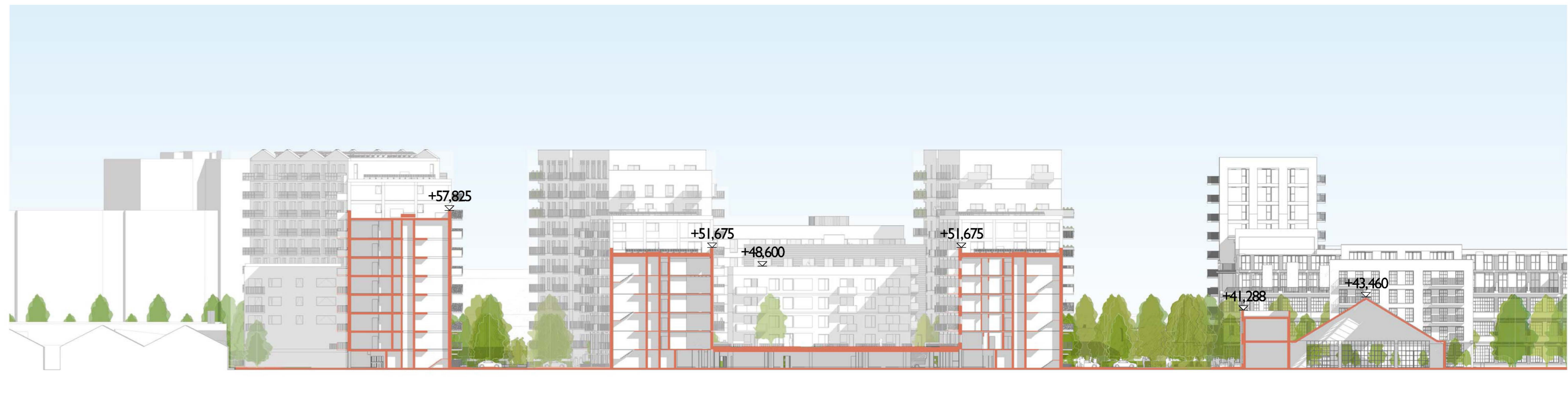
Section Transversal1 1:500
