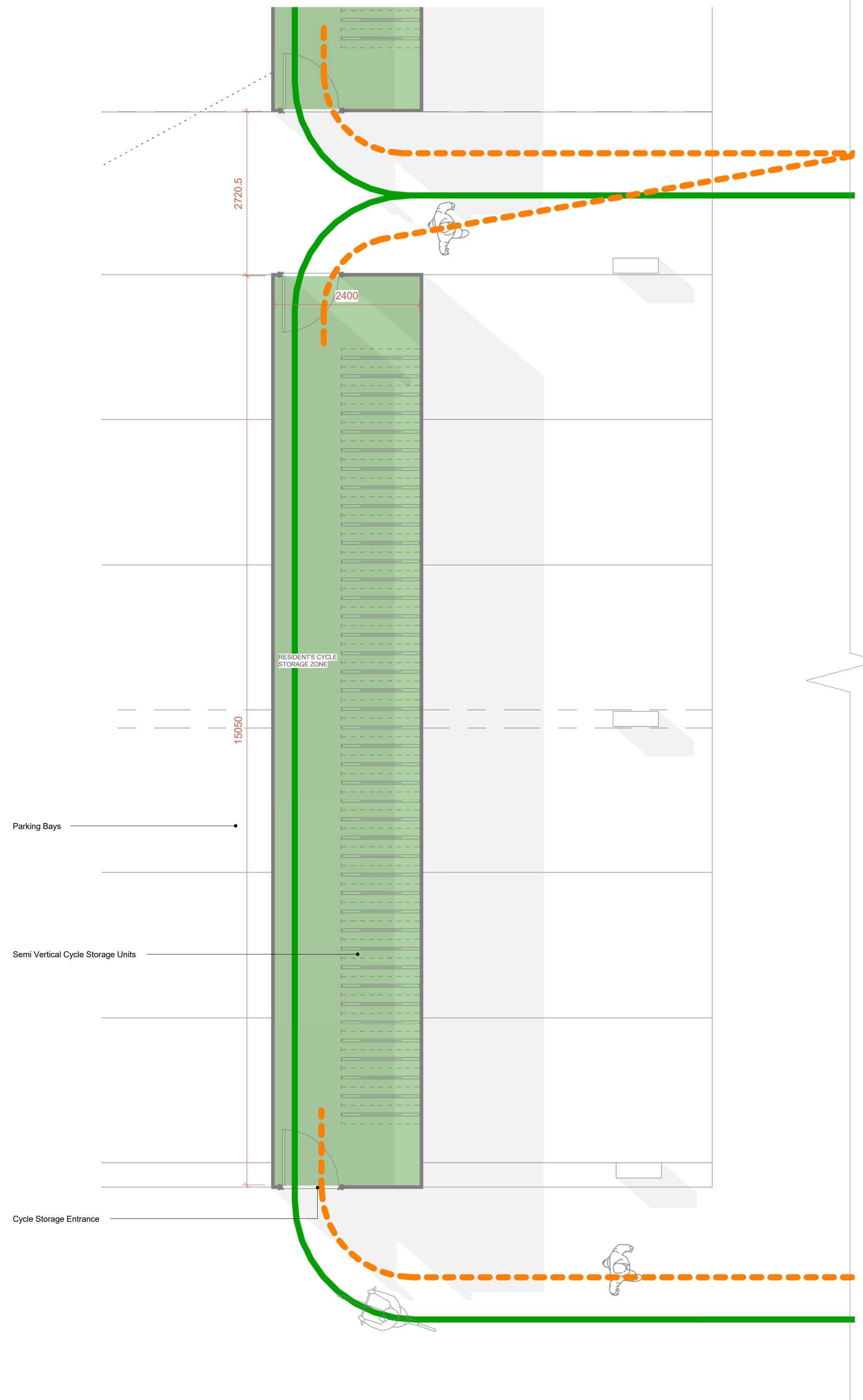
SEMI VERTICAL CYCLE STORAGE LAYOUT
