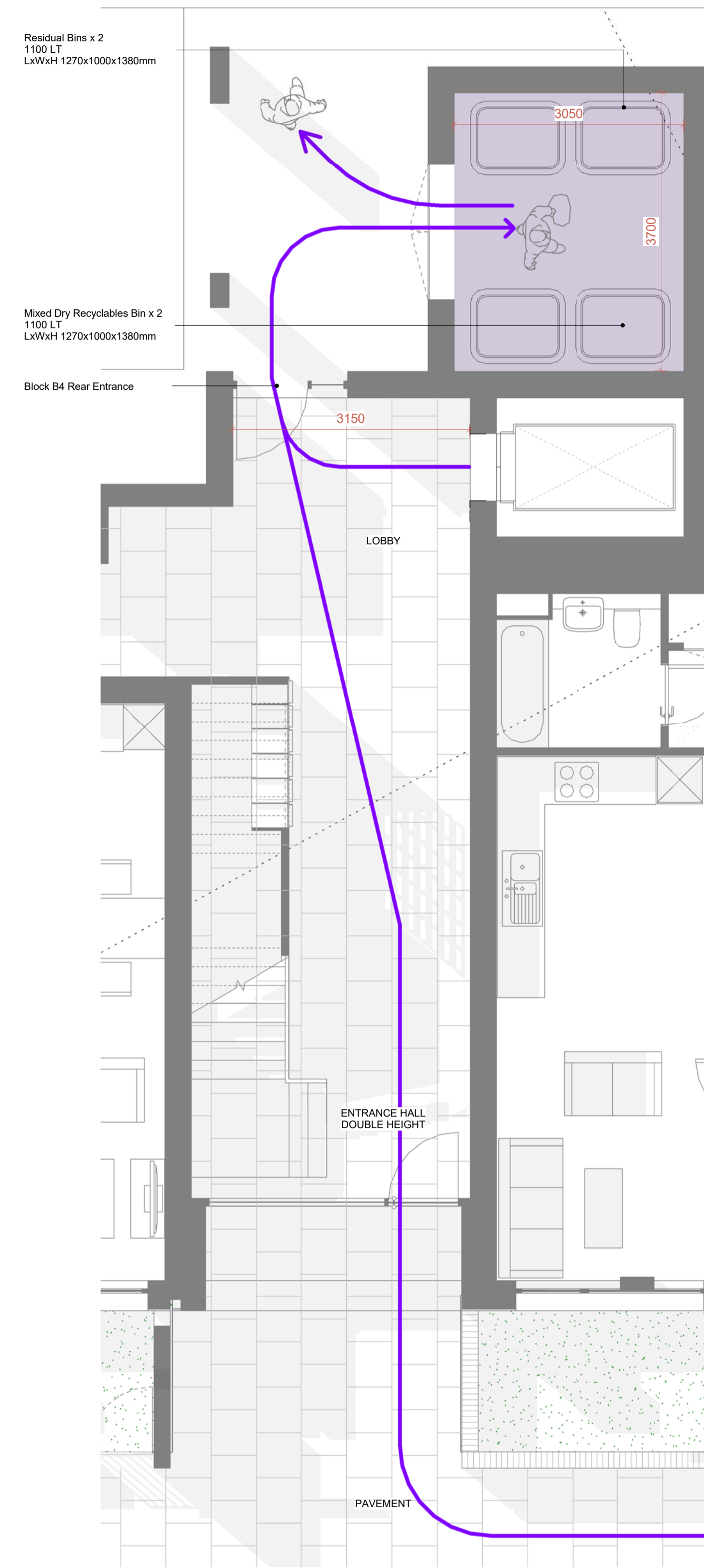
BLOCK B4 BINS LAYOUT
