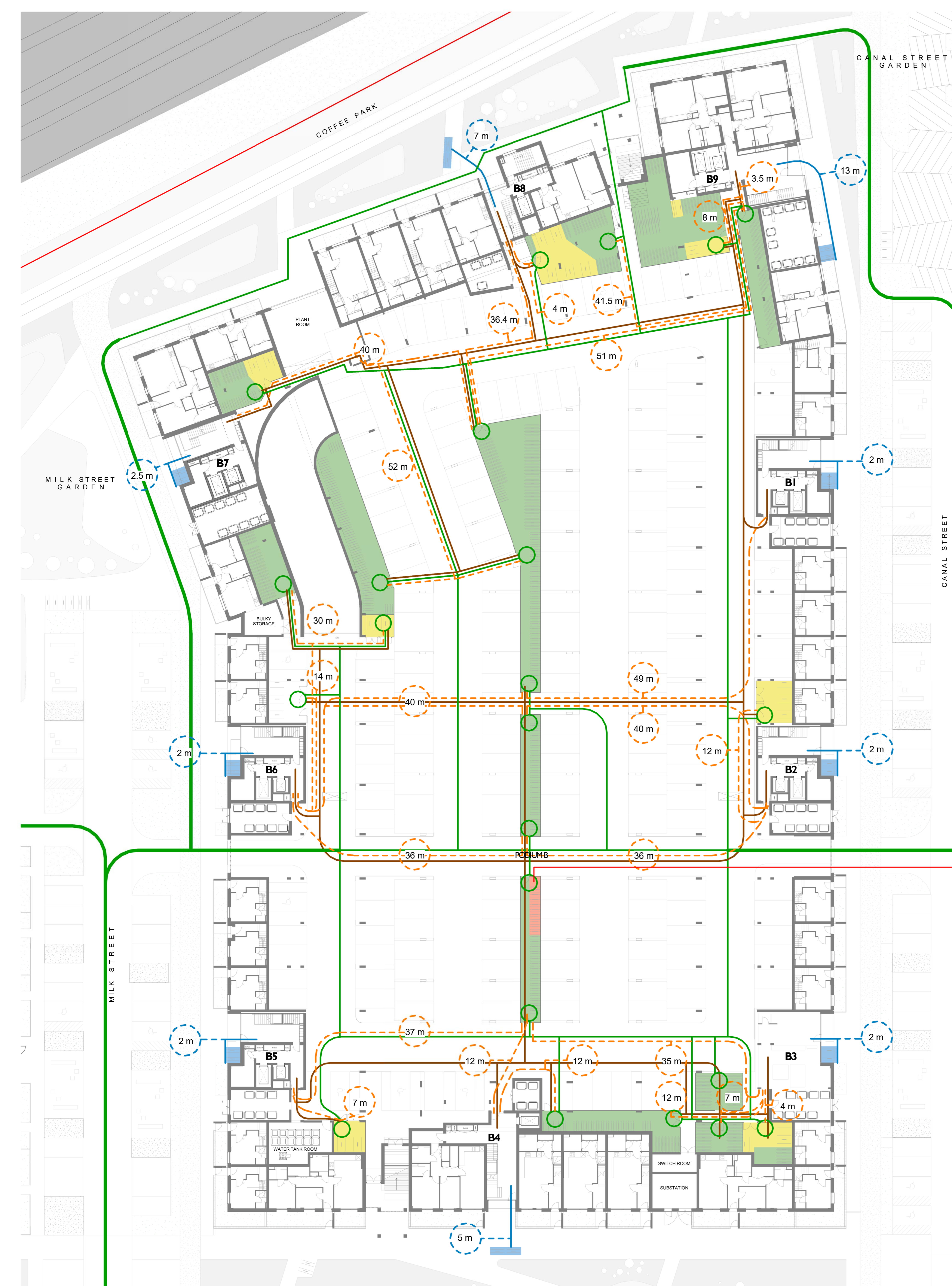
CYCLE STORAGE LAYOUT DIAGRAM
