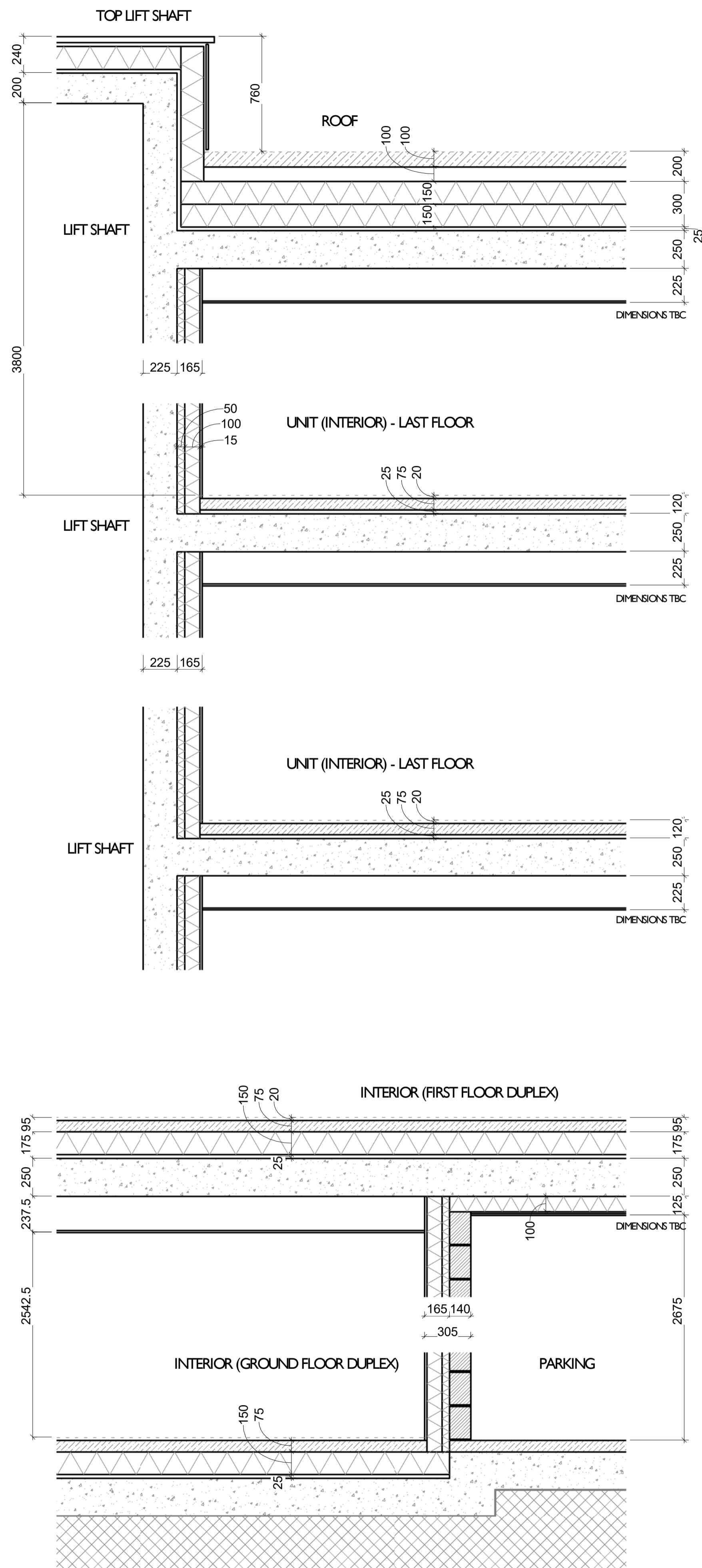
TYPICAL BUILD UP DETAIL 1 1:20
