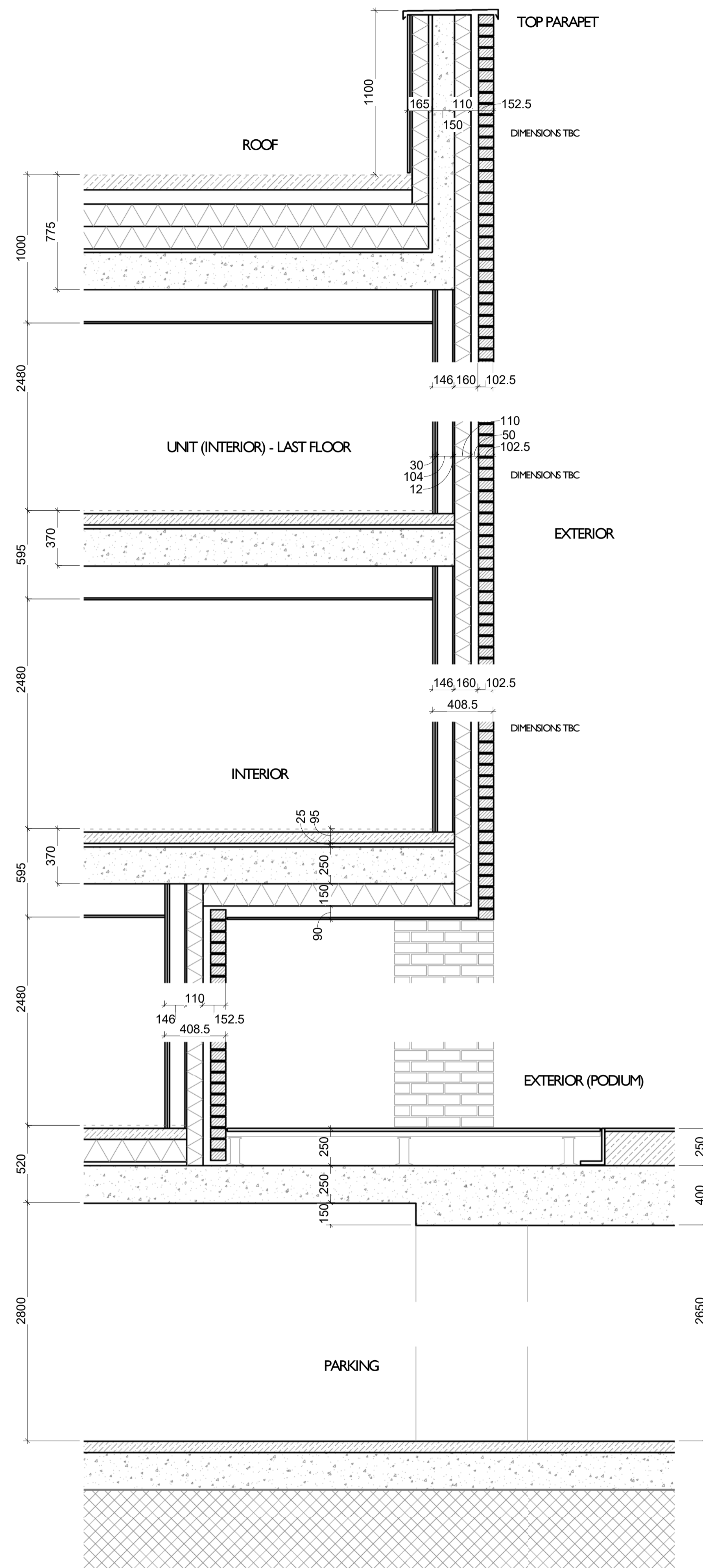
TYPICAL BUILD UP DETAIL 2 1:20
