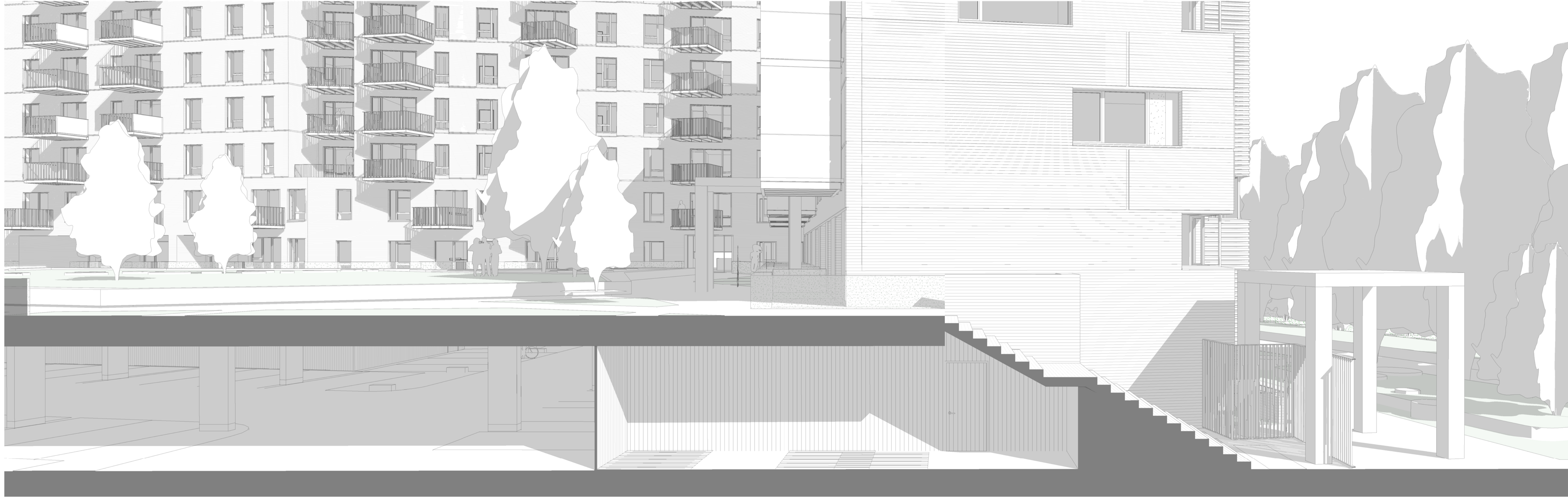
ENTRANCE PODIUM - SECTION PERSPECTIVE - SANDOW SQUARE
