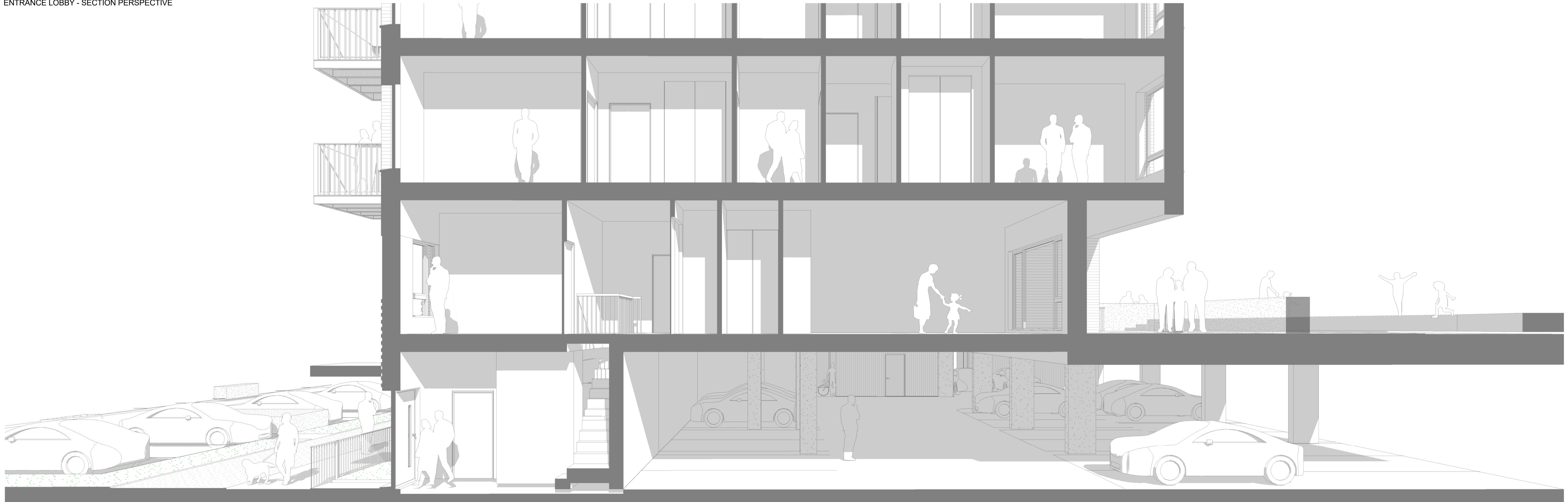
ENTRANCE DUPLEX - SECTION PERSPECTIVE
