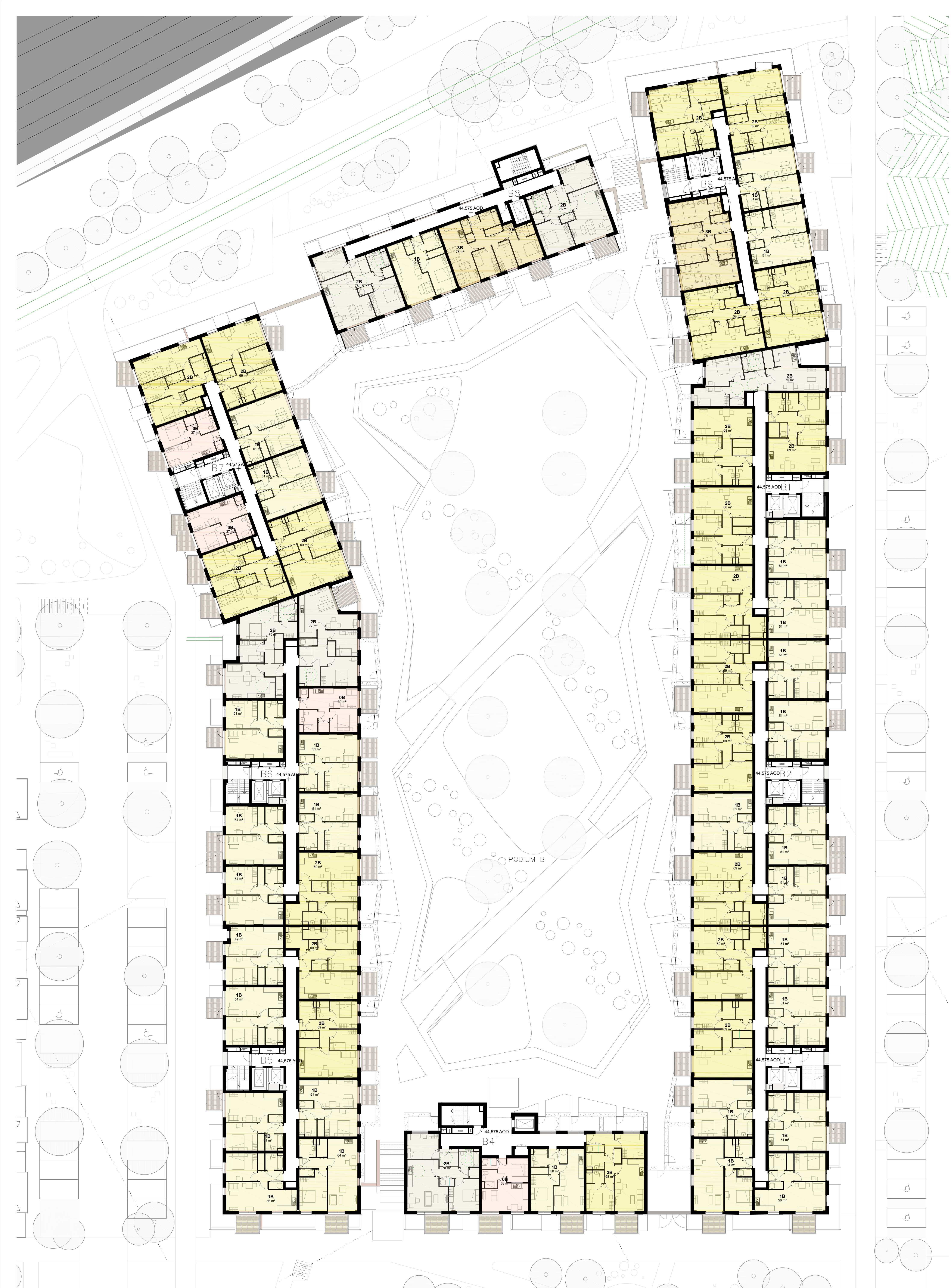
FOURTH FLOOR PLAN
