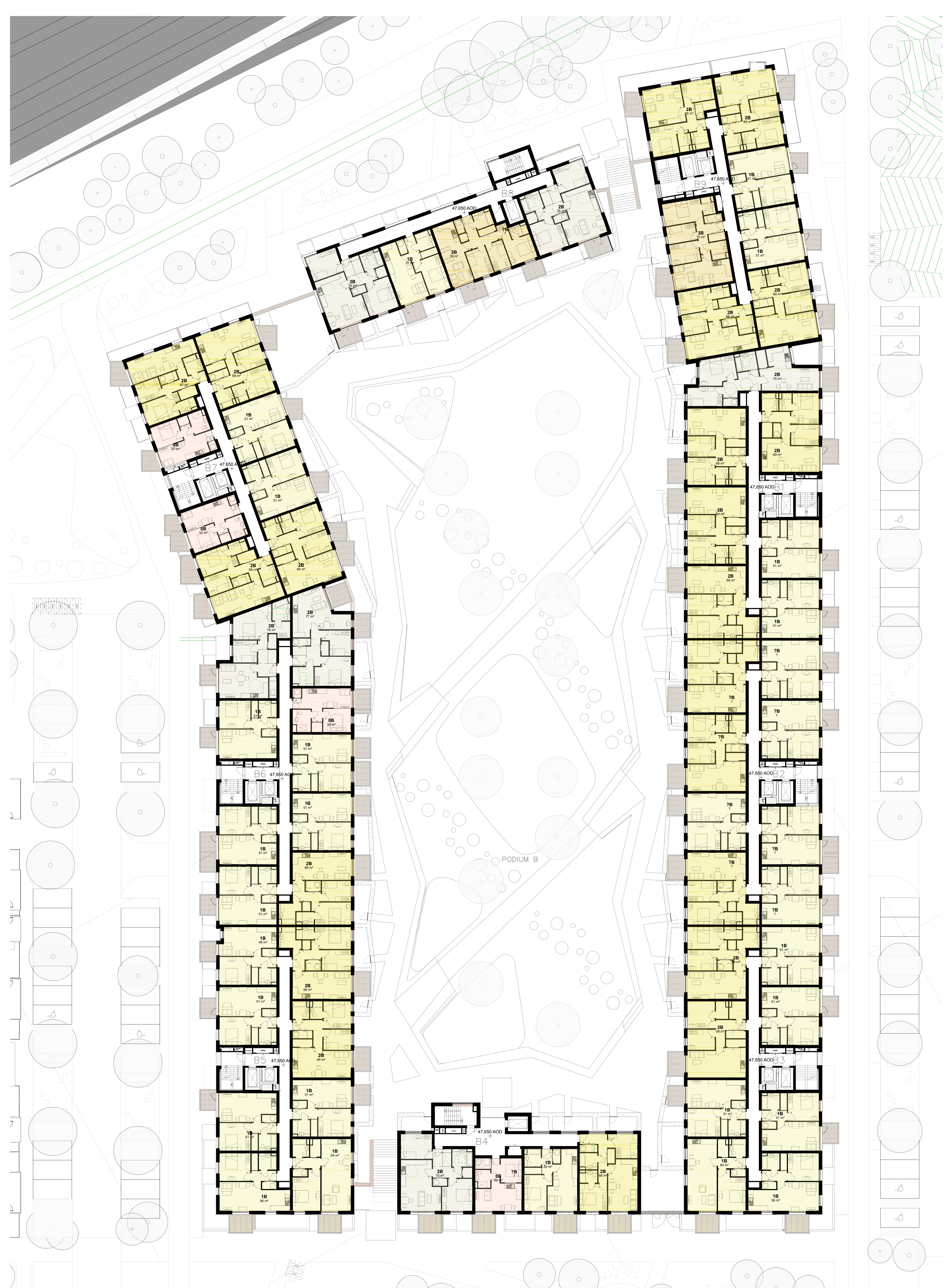
FIFTH FLOOR PLAN
