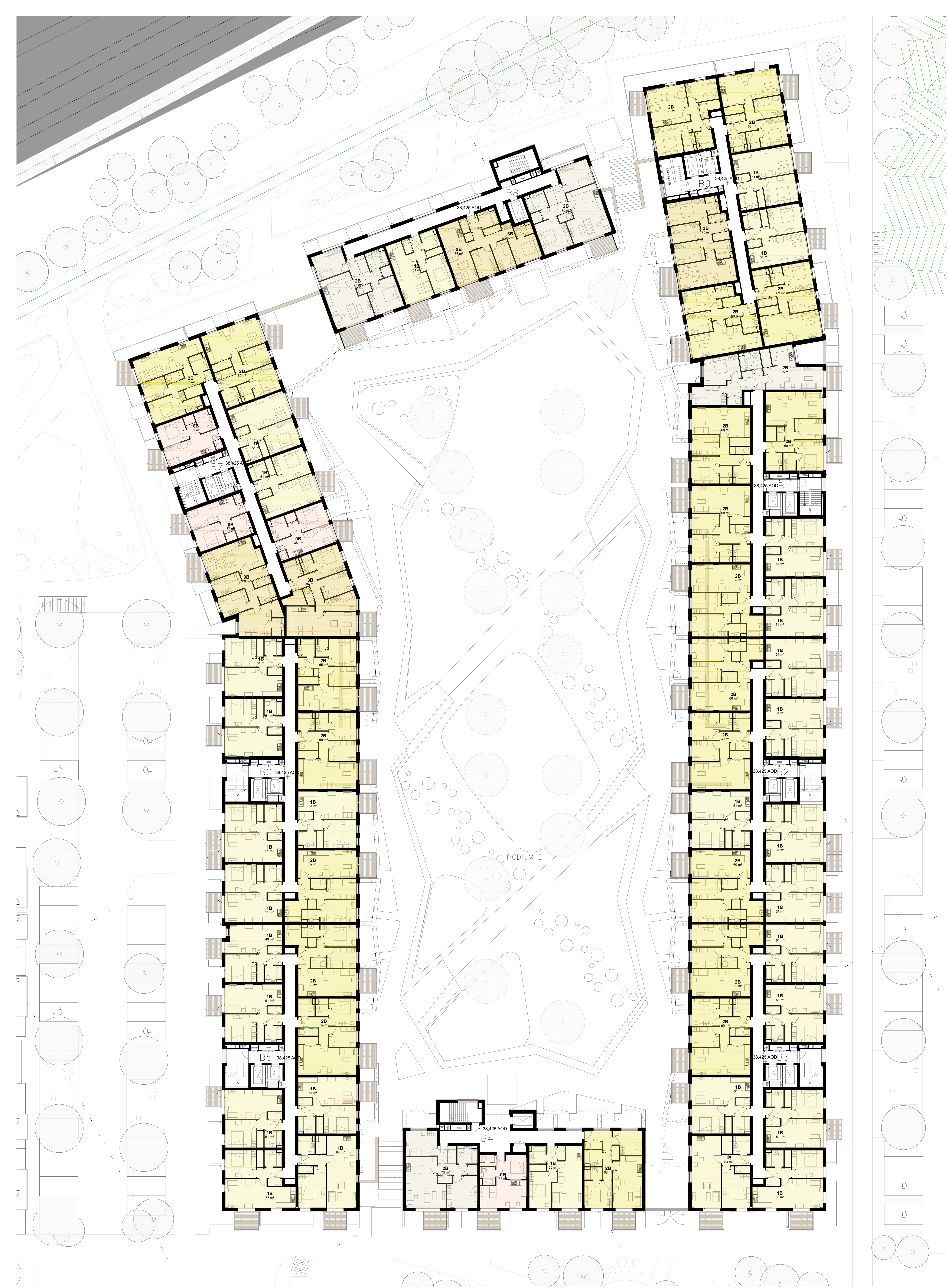
SECOND FLOOR PLAN
