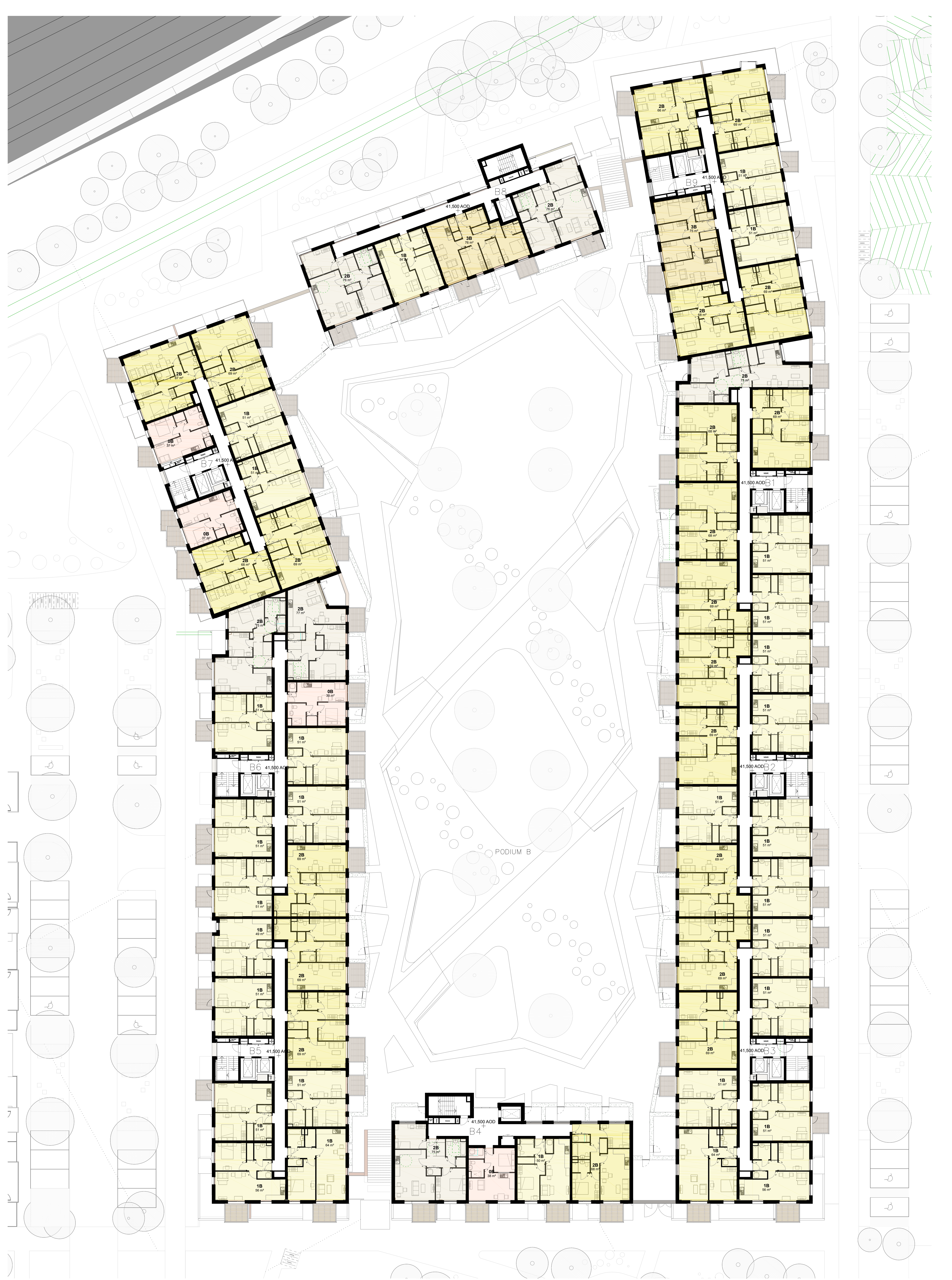
THIRD FLOOR PLAN
