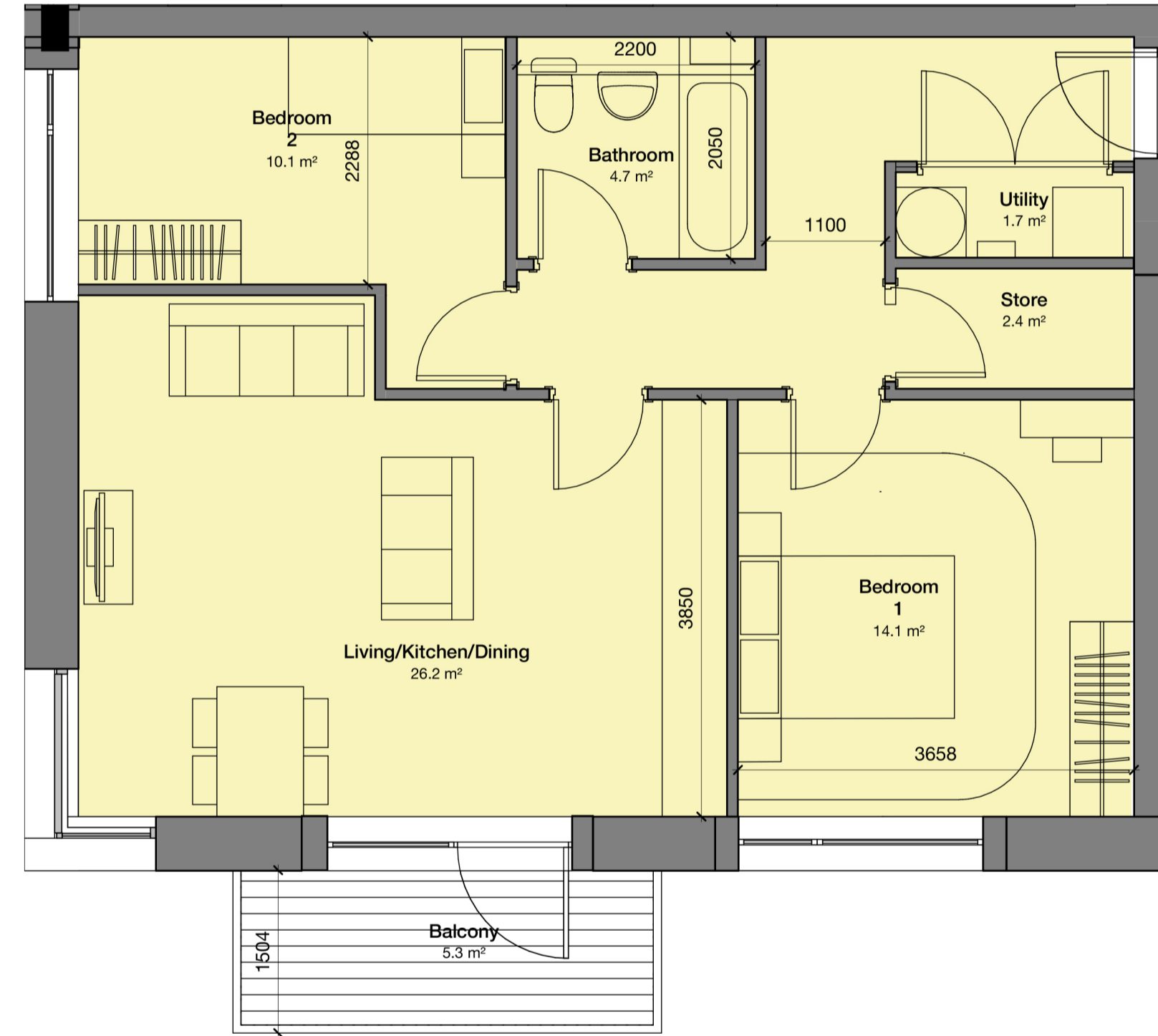
2 Bed 3 Person Flat 3 1 : 50
