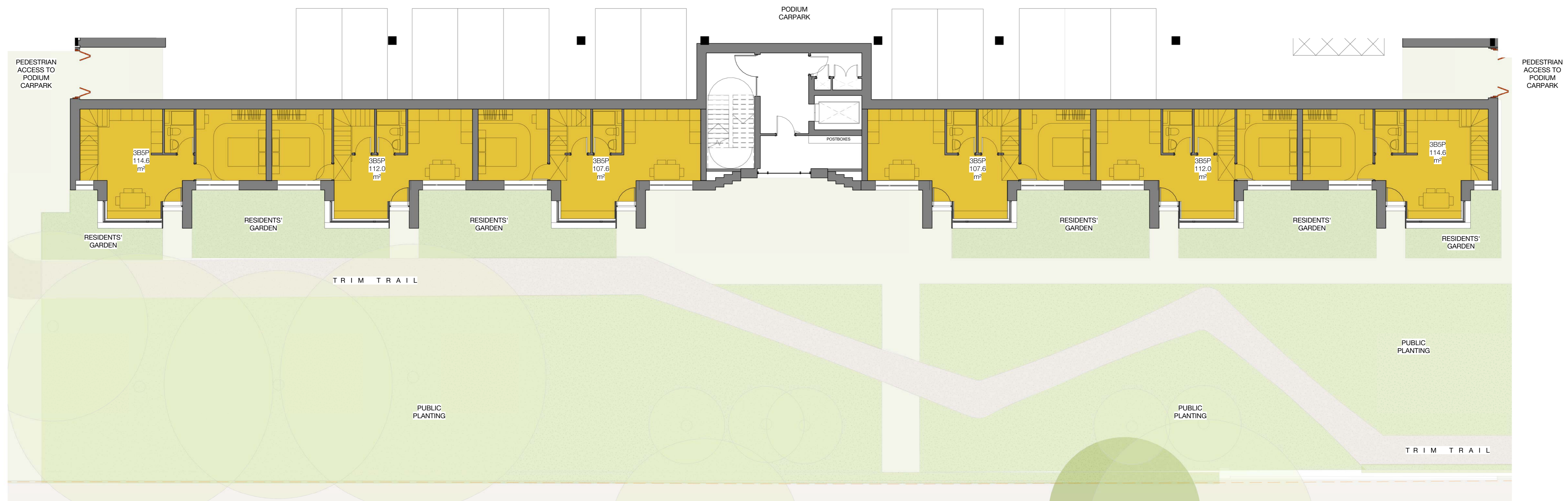
Block C6 - Ground Floor 1 : 100
