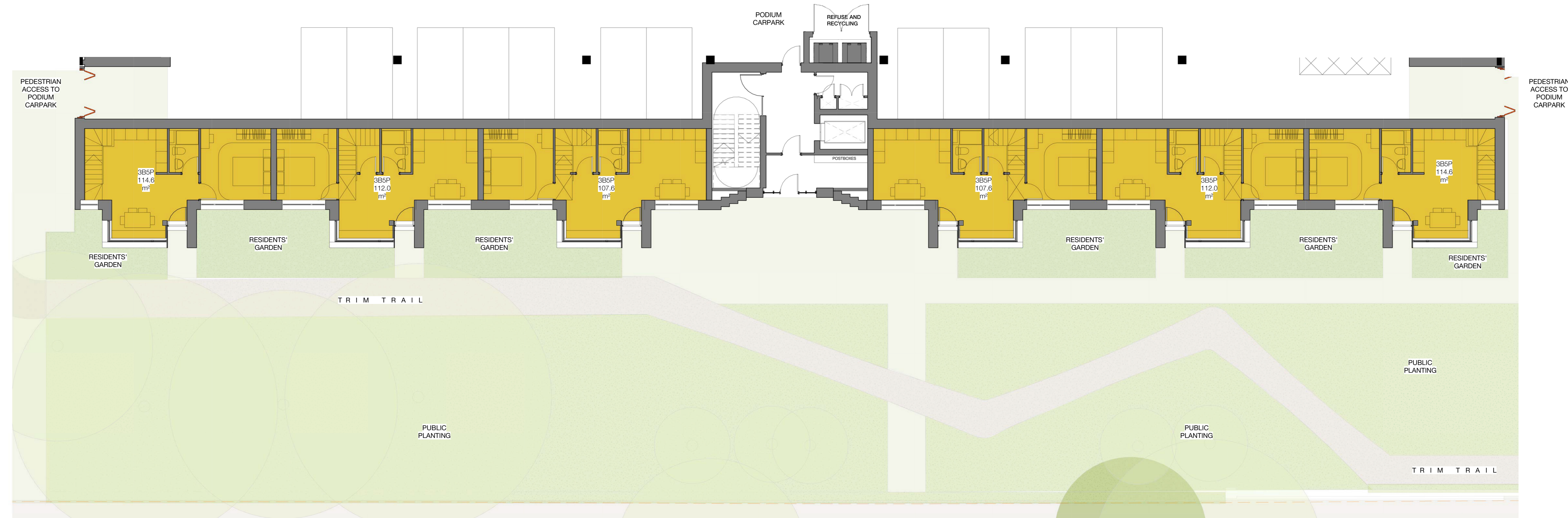
Block C6 - Ground Floor 1 : 100
