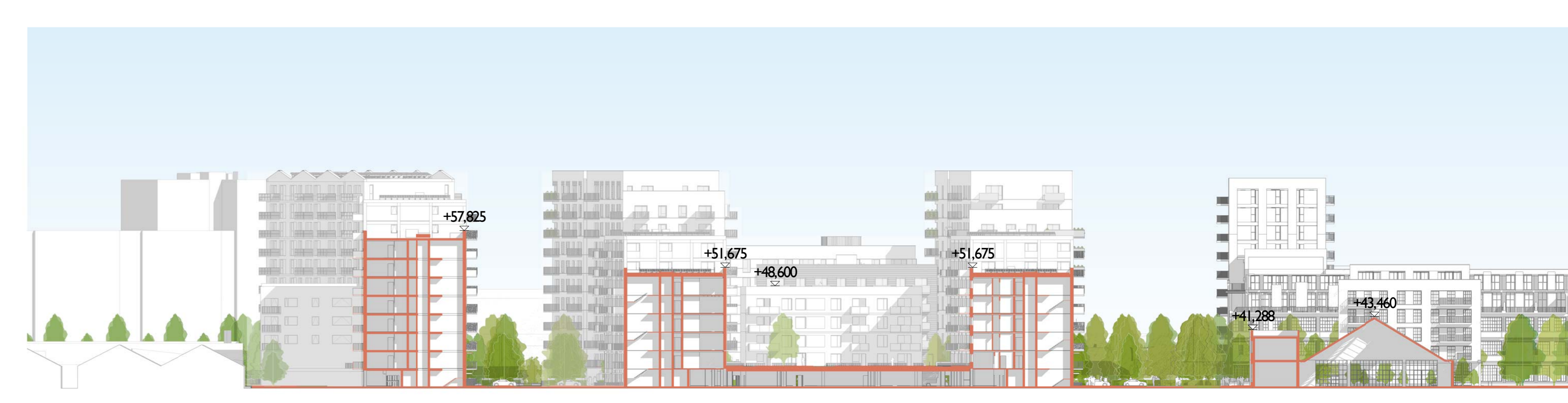
Section Transversal1 1:500
